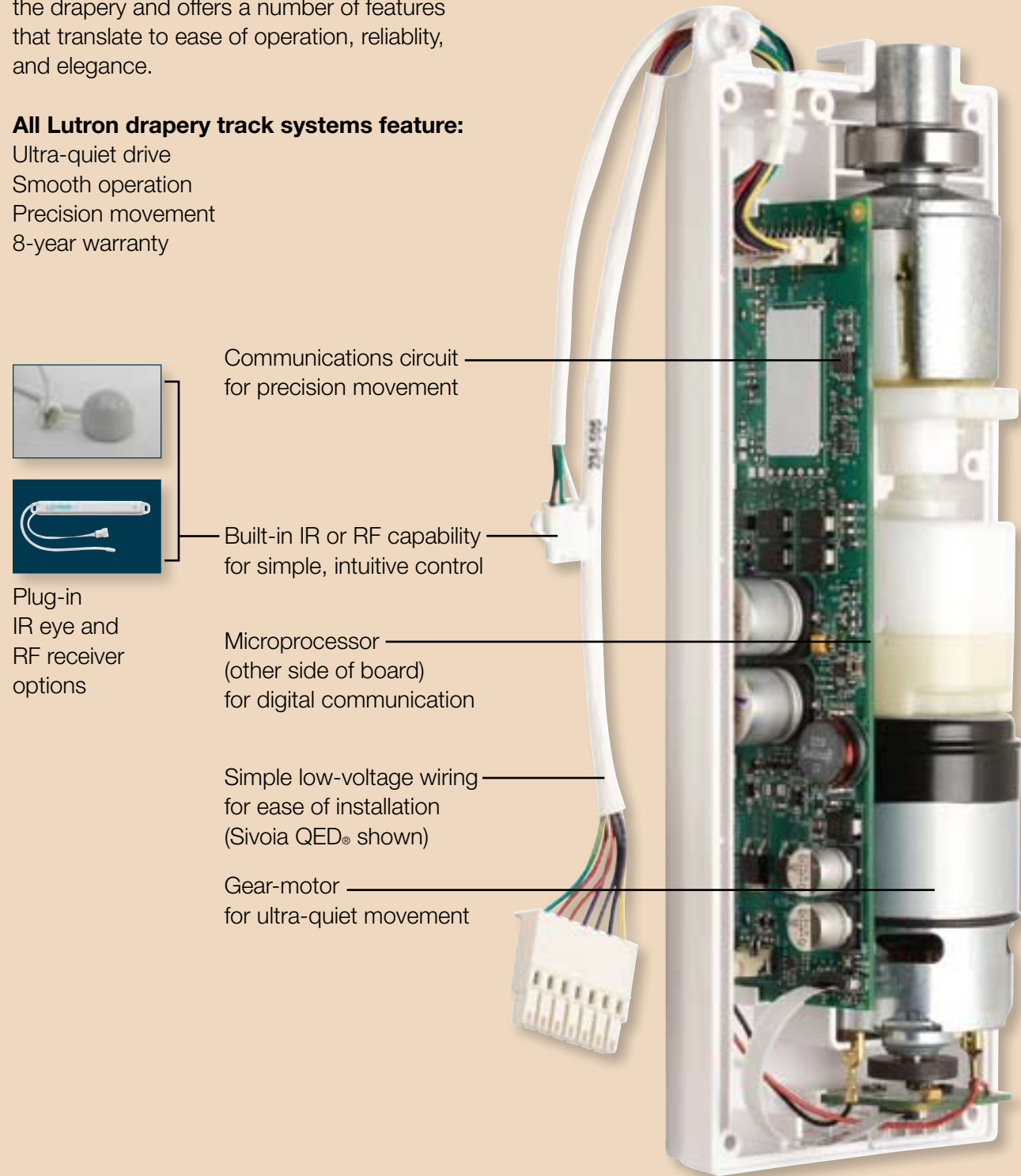
Lutron® drapery drive with cover removed
