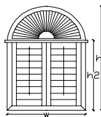
Sunburst at Top Divider Strip Frame Included in Sunburst Rail Z Frame only
